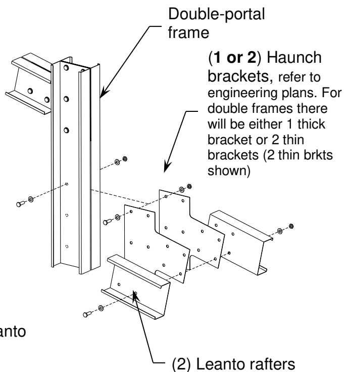
Leanto rafter to double-column assembly with drop
